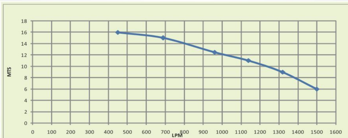
HEAD VERSUS DISCHARGE
